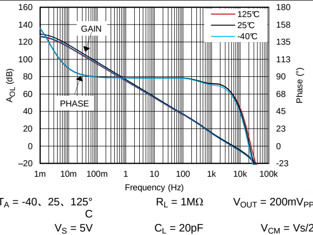
Figure 27. 开环增益和相位, 5V, 1MΩ 负载
