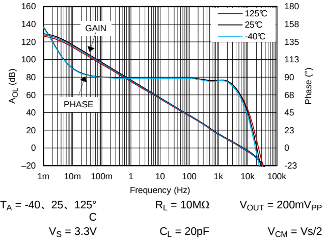
Figure 26. 开环增益和相位, 3.3V, 10MΩ 负载
