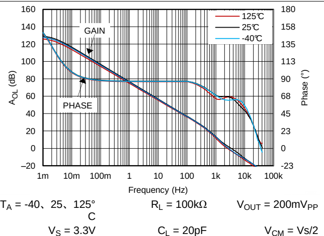
Figure 30. 开环增益和相位, 3.3V, 100kΩ 负载
