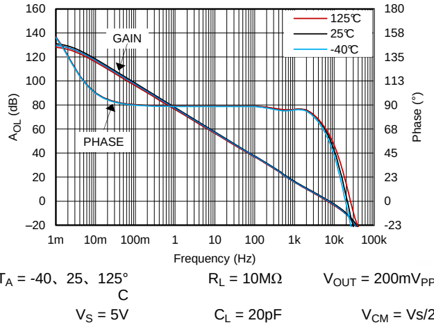
Figure 25. 开环增益和相位, 5V, 10MΩ 负载
