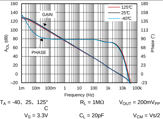
Figure 28. 开环增益和相位, 3.3V, 1MΩ 负载
