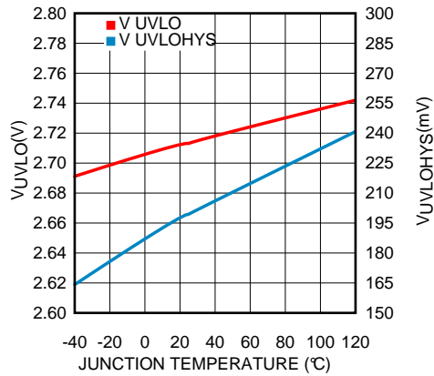
Figure 7. UVLO Threshold and Hysteresis vs Temperature
