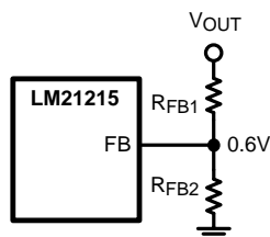
Figure 24. Setting V_{OUT}
