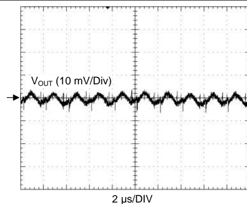
Figure 35. Output Voltage Ripple ( I_{\text{OUT}} = 15 A)
