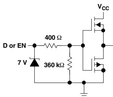
DRIVER INPUT AND ACTIVE-HIGH ENABLE
