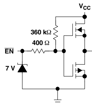
ACTIVE-LOW ENABLE
