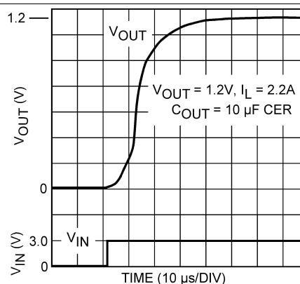
Figure 27. Turnon Time
