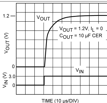
Figure 26. Turnon Time
