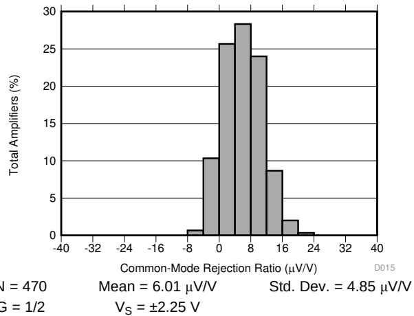
图 15. Typical CMRR Distribution
