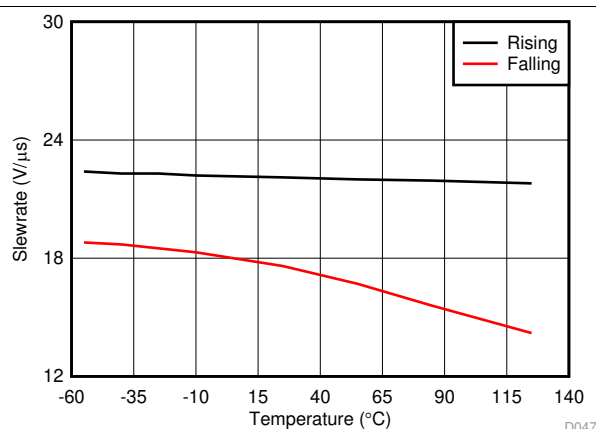
图 47. Slew Rate Over Temperature
