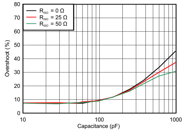
图 50. Small-Signal Overshoot vs Capacitive Load
