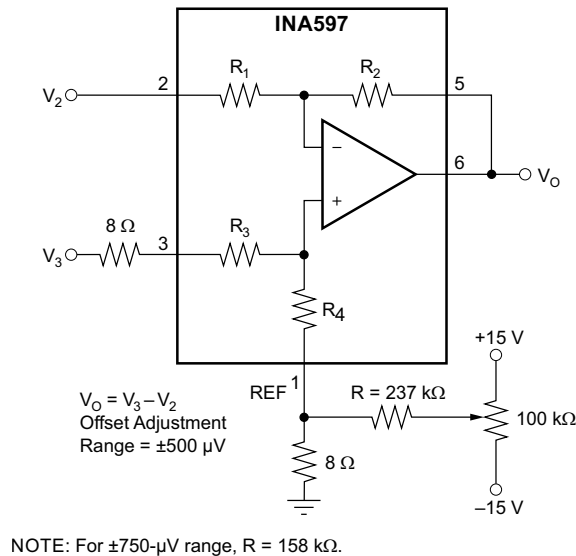
图 75. Offset Adjustment
