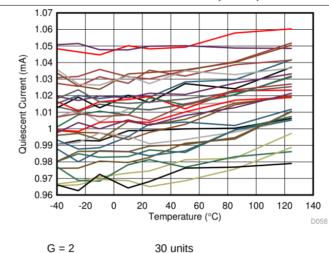
图 58. Supply Current vs Temperature
