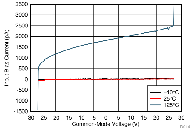
图 14. Input Bias Current vs Common-Mode Voltage
