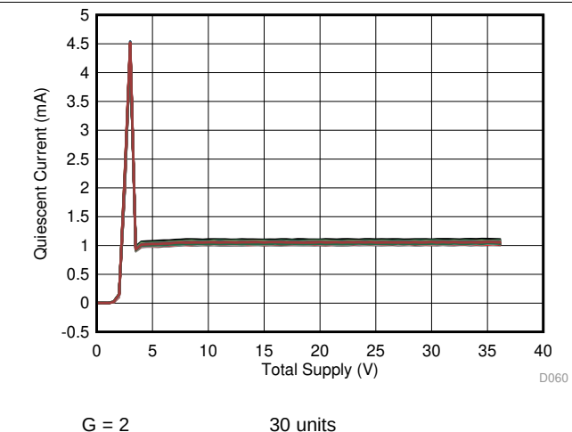
图 60. Supply Current vs Supply Voltage
