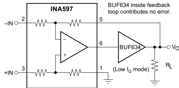
图 79. Low Power, High-Output Current, Precision, Difference Amplifier
