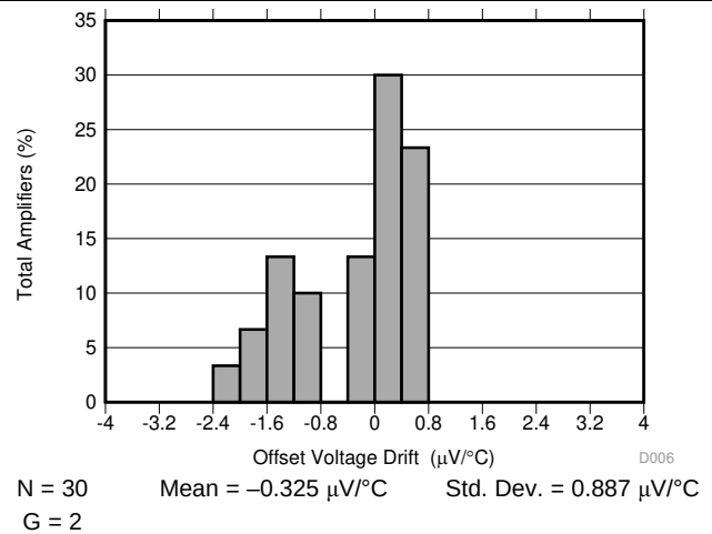
图 6. Typical Distribution of Offset Voltage Drift (RTO)
