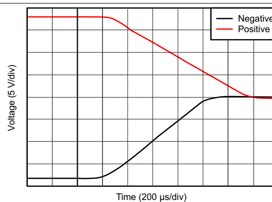
图 46. Large-Signal Step Response
