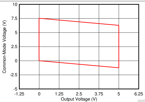
图 68. Input Common-Mode Voltage vs Output Voltage
