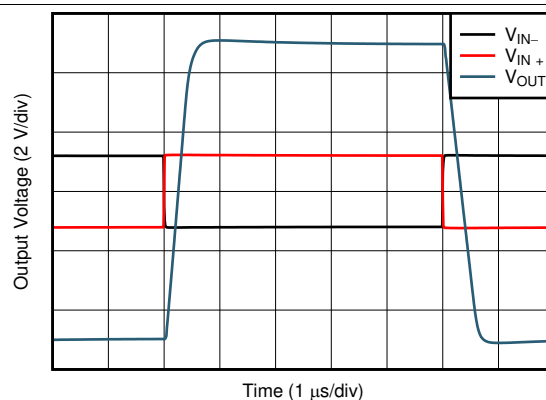
图 44. Settling Time
