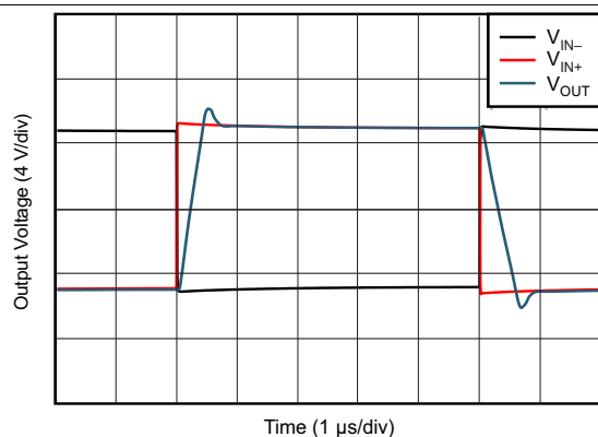
图 43. Settling Time
