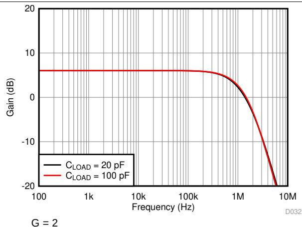
图 32. Closed-Loop Gain vs Frequency
