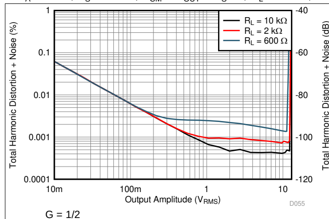
图 55. THD+N Ratio vs Output Amplitude
