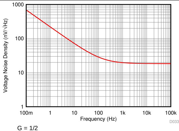
图 33. Voltage Noise Spectral Density vs Frequency (RTI)
