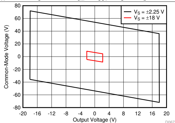
图 67. Input Common-Mode Voltage vs Output Voltage
