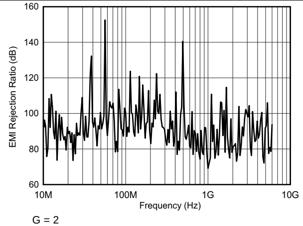
图 64. Differential-Mode EMI Rejection Ratio
