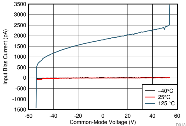
图 13. Input Bias Current vs Common-Mode Voltage
