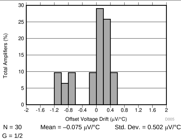
图 5. Typical Distribution of Offset Voltage Drift (RTO)
