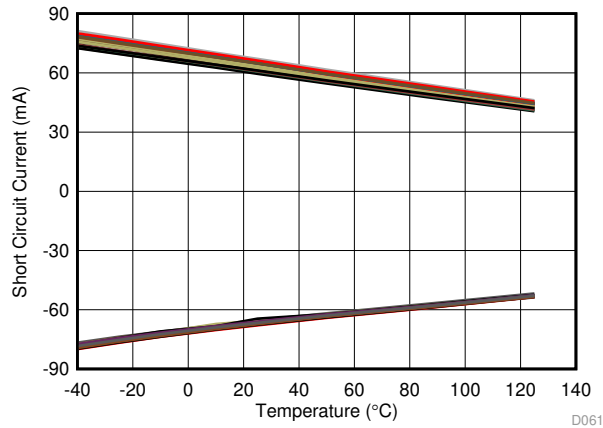
图 61. Short Circuit Current vs Temperature
