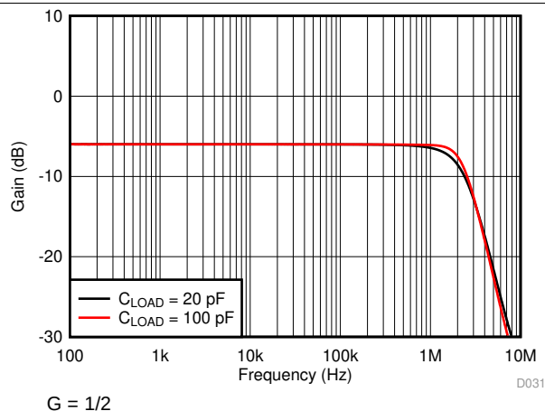
图 31. Closed-Loop Gain vs Frequency
