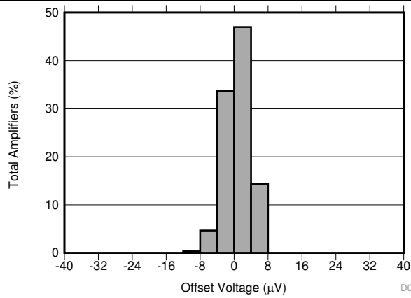
图 1. Typical Distribution of Offset Voltage (RTO)
