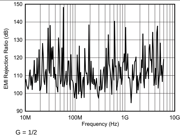
图 63. Differential-Mode EMI Rejection Ratio
