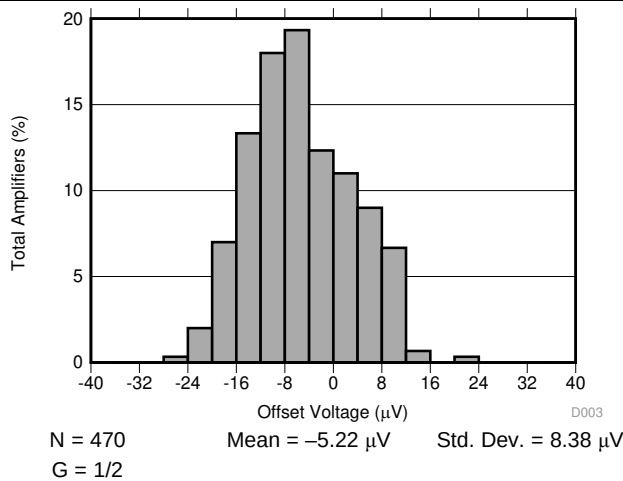
图 3. Typical Distribution of Offset Voltage (RTO)
