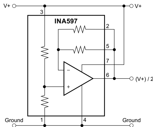
图 80. Pseudoground Generator
