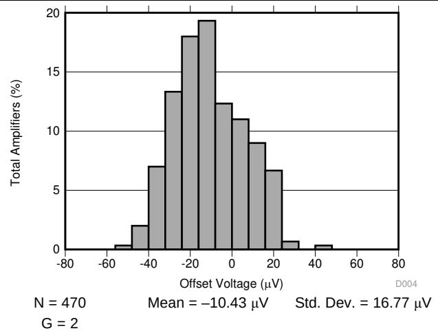
图 4. Typical Distribution of Offset Voltage (RTO)
