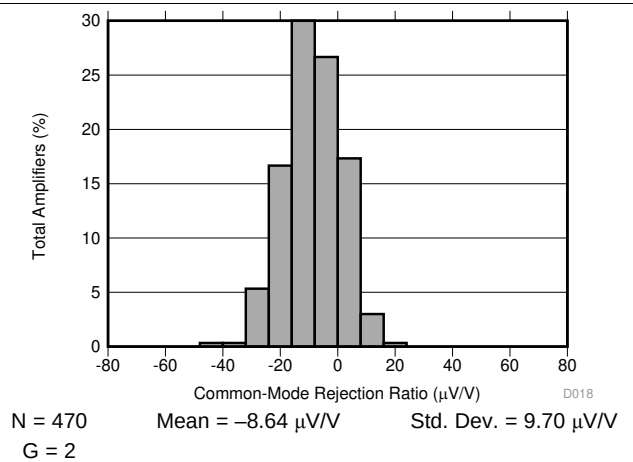
图 18. Typical CMRR Distribution
