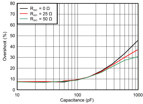
图 49. Small-Signal Overshoot vs Capacitive Load
