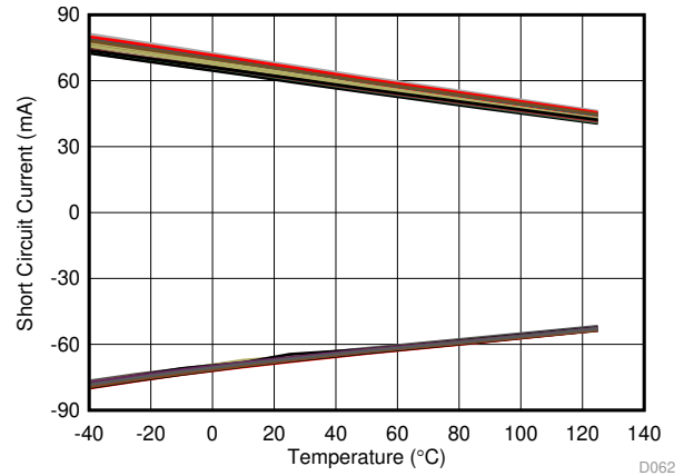
图 62. Short Circuit Current vs Temperature
