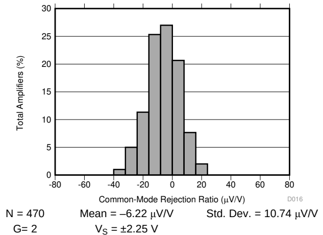
图 16. Typical CMRR Distribution ,
