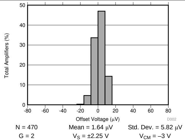
图 2. Typical Distribution of Offset Voltage (RTO)
