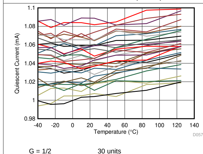
图 57. Supply Current vs Temperature
