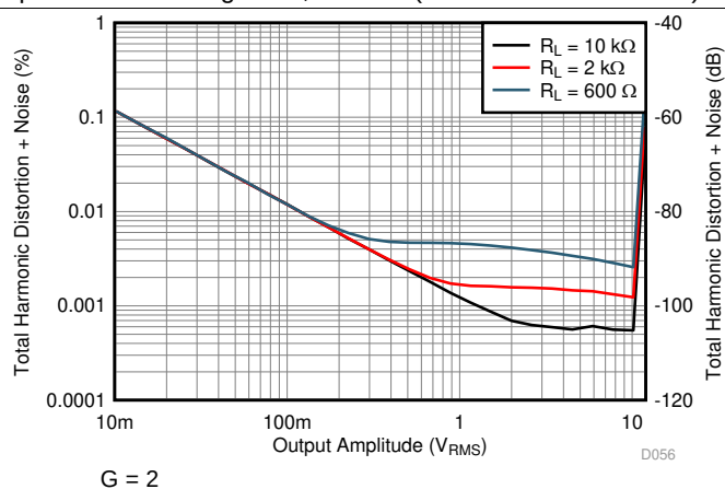
图 56. THD+N Ratio vs Output Amplitude
