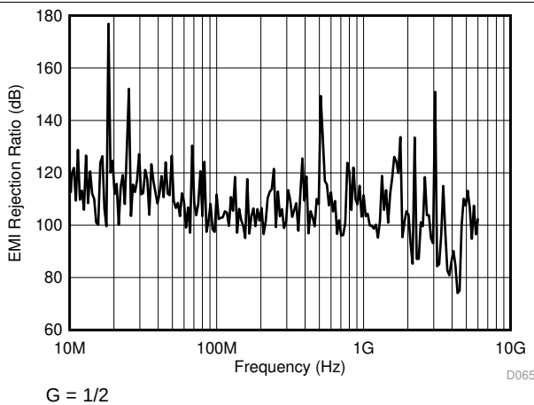
图 65. Common-Mode EMI Rejection Ratio
