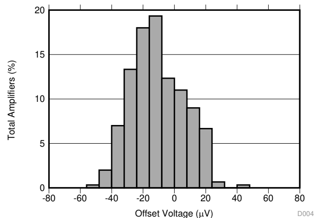
失调电压的典型分布 (RTO) G = 1/2, V S = ±18V
