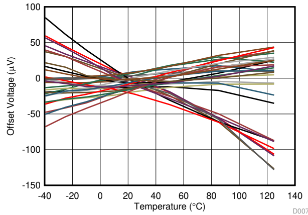
图 7. Output Offset Voltage vs Temperature
