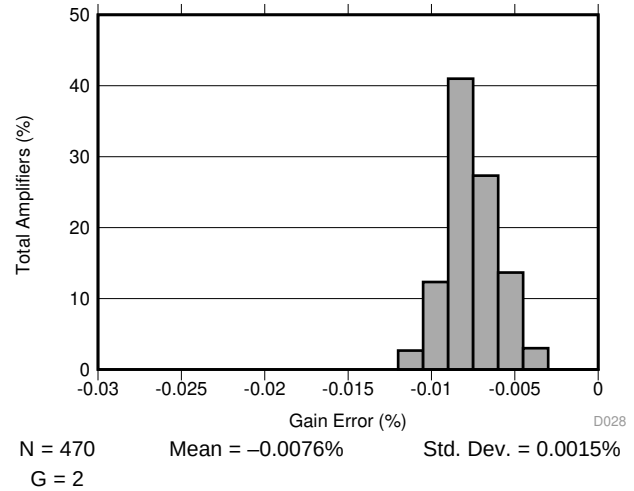
图 28. Typical Distribution of Gain Error
