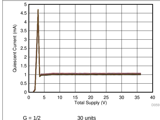
图 59. Supply Current vs Supply Voltage
