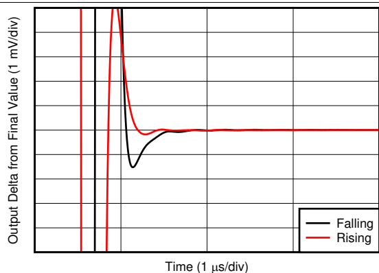
图 43. Settling Time
