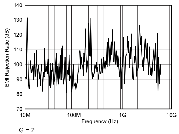
图 66. Common-Mode EMI Rejection Ratio
