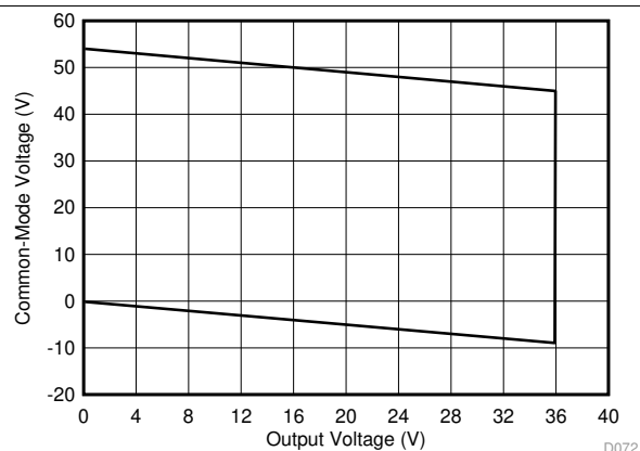
图 70. Input Common-Mode Voltage vs Output Voltage ,
