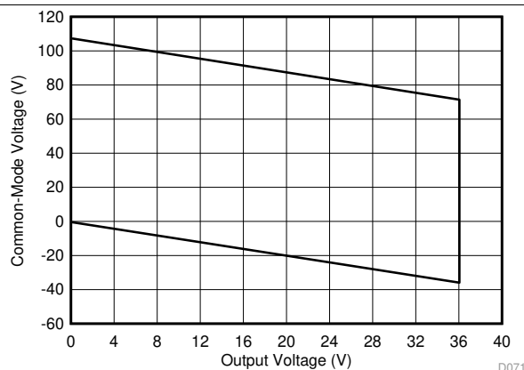
图 69. Input Common-Mode Voltage vs Output Voltage
