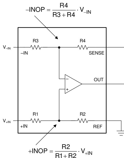
图 76. Voltage Division in the Difference Amplifier Configuration
