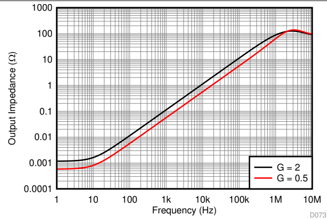
图 73. Closed-Loop Output Impedance vs Frequency
