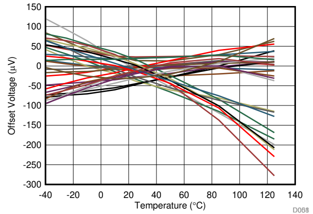
图 8. Output Offset Voltage vs Temperature
