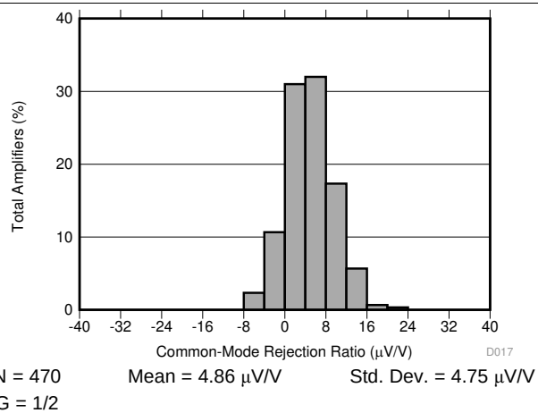
图 17. Typical CMRR Distribution
