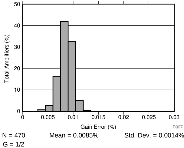
图 27. Typical Distribution of Gain Error
