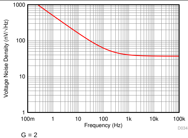
图 34. Voltage Noise Spectral Density vs Frequency (RTI)
