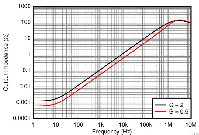
图 77. Closed-Loop Output Impedance vs Frequency
