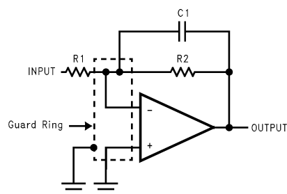
Figure 32. Inverting Amplifier
