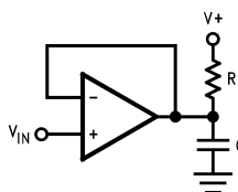
Figure 30. Compensating for Large Capacitive Loads with a Pull Up Resistor
