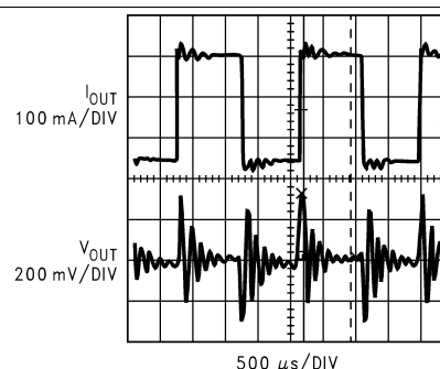
Figure 18. 130-mA to 400-mA Transient Response of the Circuit in Figure 24 With C_{FF} Disconnected
