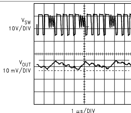
Figure 20. Pulse-Skipping Mode
