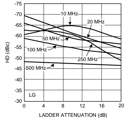
Figure 22. HD2 vs Ladder Attenuation
