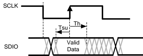
Figure 57. Write Timing
