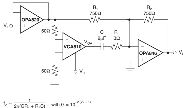
Figure 43. Tunable Equalizer
