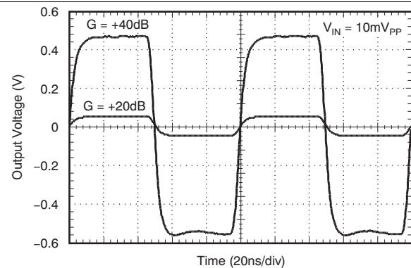
Figure 4. High Gain Pulse Response
