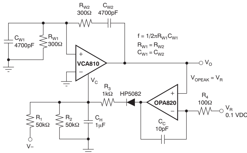
Figure 38. Amplitude-Stabilized Oscillator
