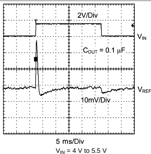
Figure 10. Line Transient Response
