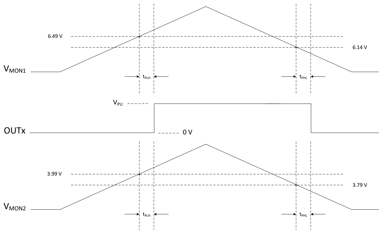
Figure 24. Overvoltage Detection
