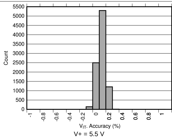
Figure 6. INx Threshold ( V_{IT-} )
