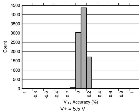
Figure 5. INx Threshold ( V_{IT+} )
