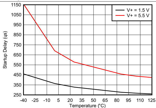
Figure 15. Startup Delay
