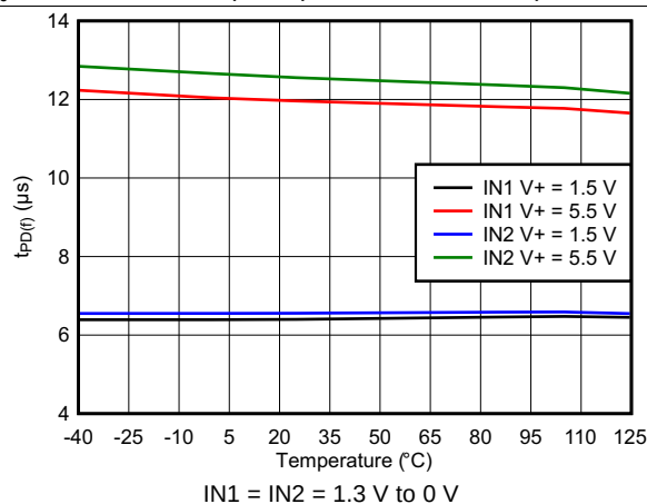
Figure 14. Propagation Delay from INx Low to Output Low
