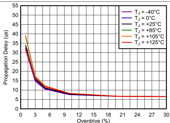
Figure 14. Propagation Delay from INx Low to Output Low
