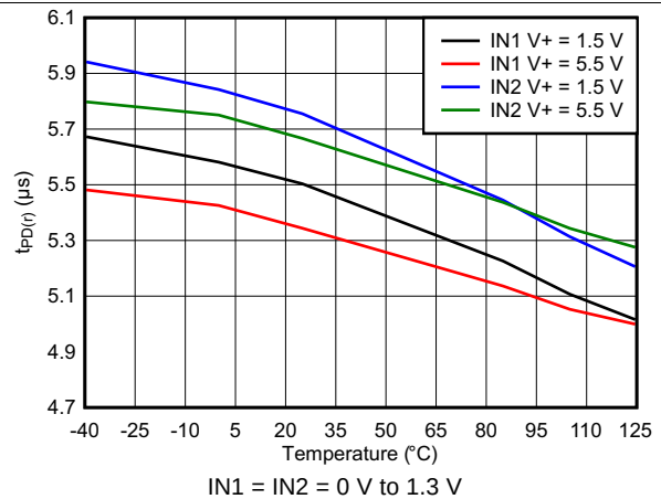
Figure 13. Propagation Delay from INx High to Output High
