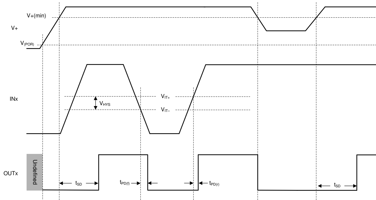
Figure 1. Timing Diagram
