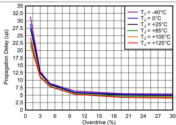
Figure 17. Propagation Delay vs Overdrive ( V+ = 5.5\text{ V} )
