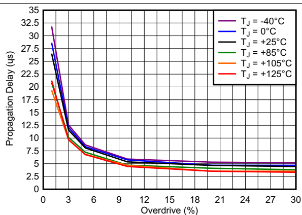
Figure 16. Propagation Delay vs Overdrive ( V+ = 1.5\text{ V} )
