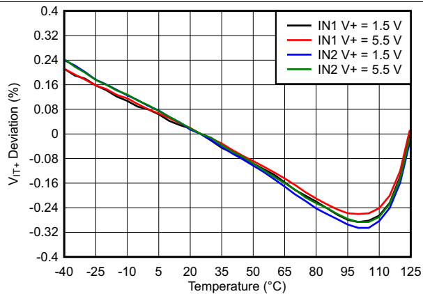
Figure 3. INx Threshold ( V_{IT+} ) Deviation vs Temperature
