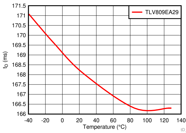
图 22. Reset Delay Time Over Temperature for TLV809EA29
