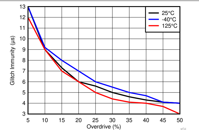
图 27. Glitch Immunity Versus Overdrive for TLV803EA29
