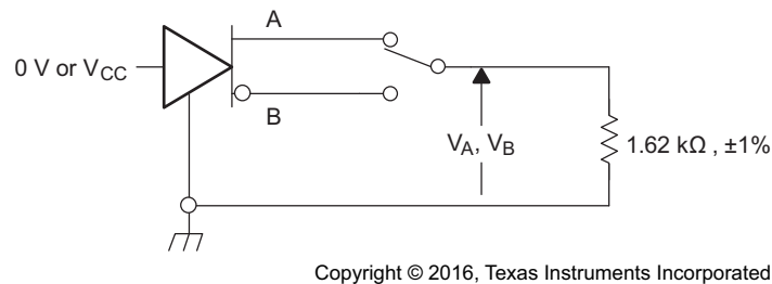
图 8. Maximum Steady State Output Voltage
