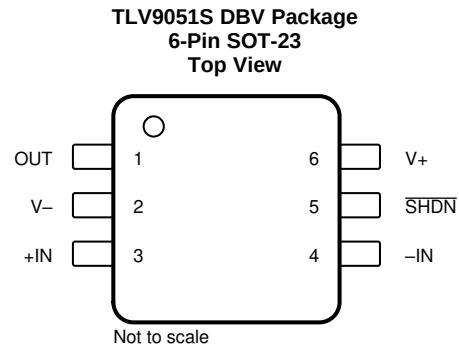
Pin Functions: TLV9051S
