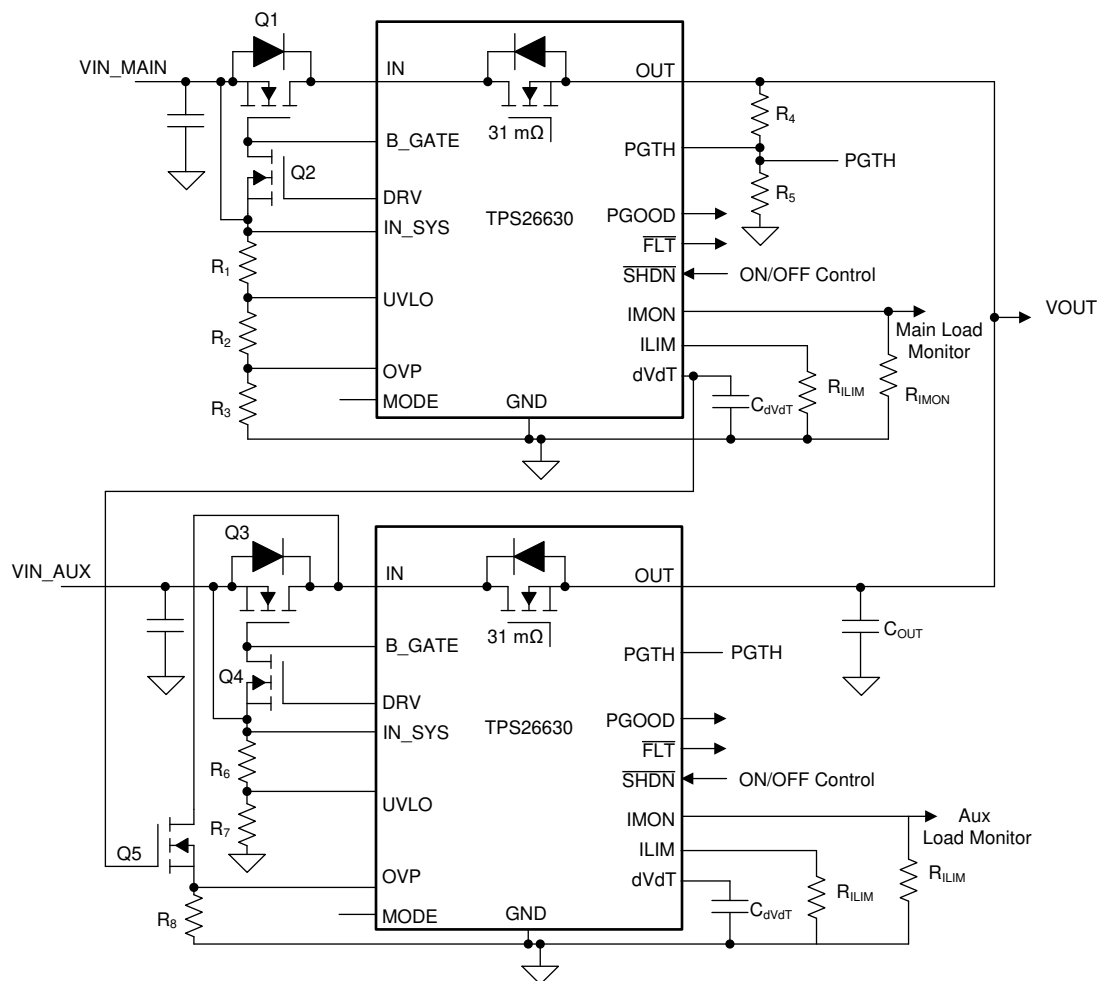
图 53. Priority Power Mux Implementation
