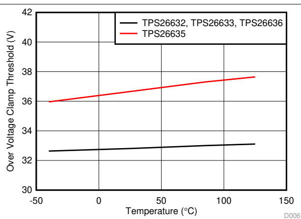
图 2. Overvoltage Clamp Threshold vs Temperature
