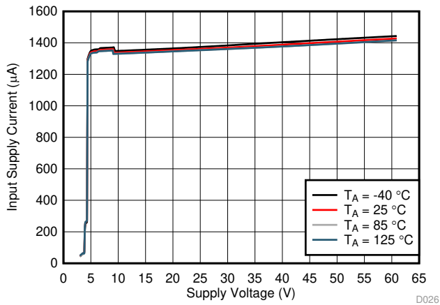
图 7. Input Supply Current vs Supply Voltage During Normal Operation
