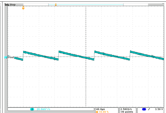
Figure 36. TPS62745 with V_{OUT} = 3.3\text{ V} ; Output Voltage Ripple for I_{OUT} = 1\text{ mA}
