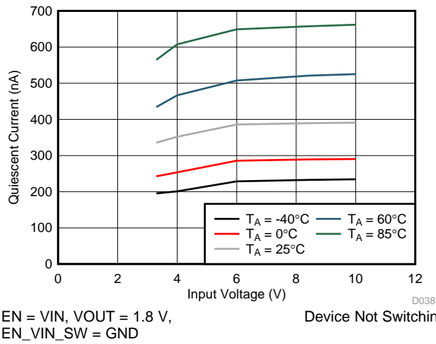
Figure 1. Quiescent Current
