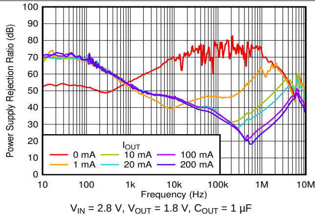
图 43. PSRR vs Frequency and I_{OUT}
