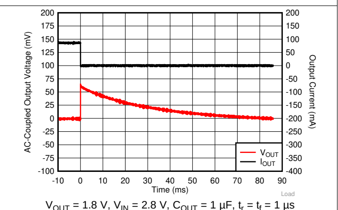
图 18. I_{OUT} Transient From 100 mA to 0 mA
