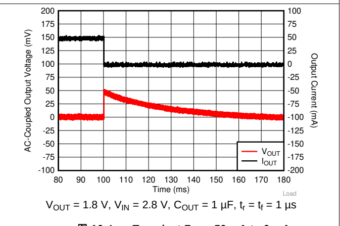
图 16. I_{OUT} Transient From 50 mA to 0 mA
