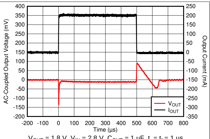
图 14. I_{OUT} Transient From 1 mA to 200 mA
