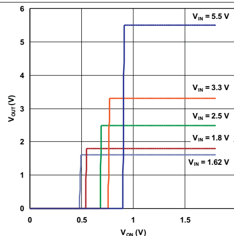
Figure 12. ON Threshold
