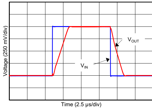
图 25. Large-Signal Pulse Response (Maximum Supply)
