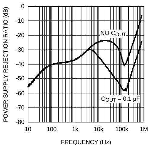
Figure 46. Power Supply Rejection vs Frequency
