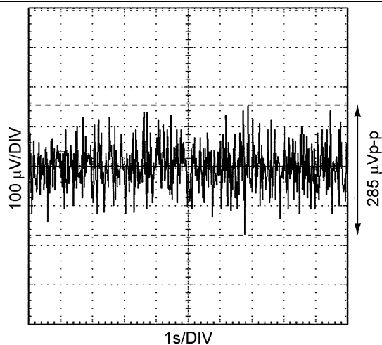
Figure 32. 0.1–10 Hz Noise
