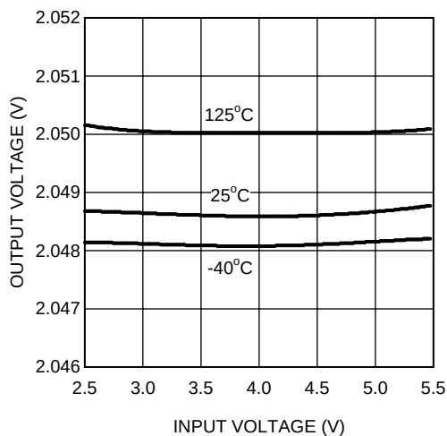
Figure 19. Line Regulation
