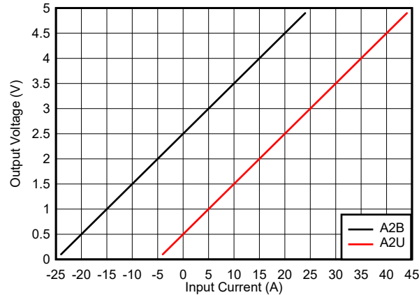
图 9-9. Output Voltage Relationship to Input Current for TMCS1107A2B-Q1 and TMCS1107A2U-Q1
