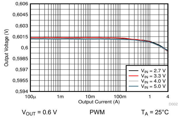
图 10-21. Output Voltage versus Output Current
