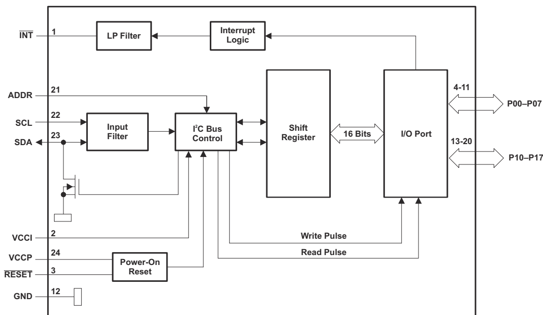
图 8-1. Logic Diagram (Positive Logic)
