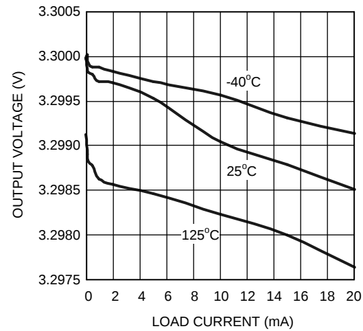
Figure 36. Load Regulation
