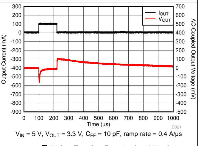
图 10. I_{OUT} Transient From 0 mA to 100 mA
