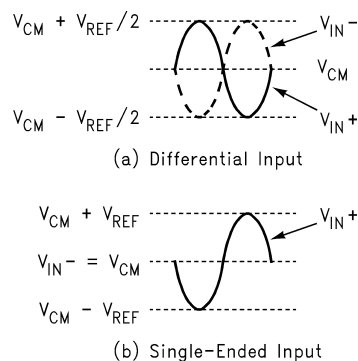
Figure 23. Expected Input Signal Range
