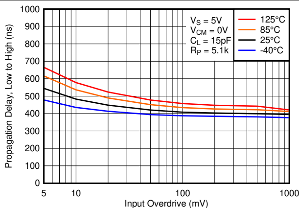
图 7-31. Low to High Propagation Delay vs. Input Overdrive Voltage, 5V
