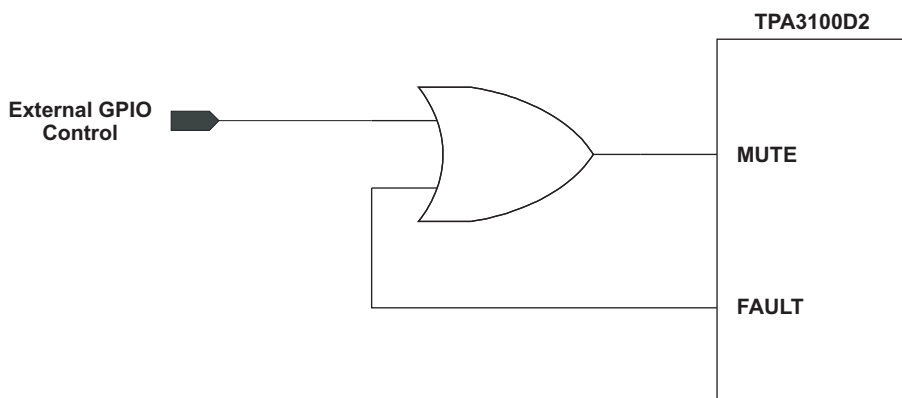
Figure 34. External MUTE Control
