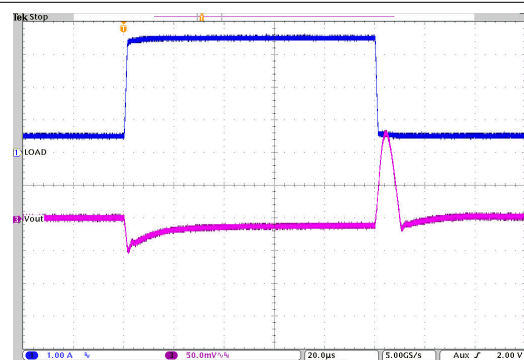
图 10-29. Load Transient Response
