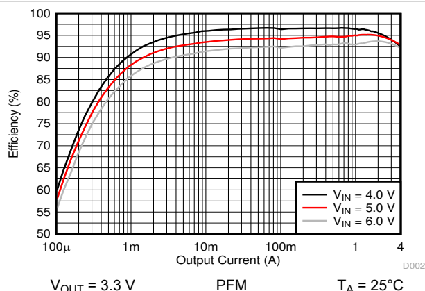
图 10-2. Efficiency versus Output Current
