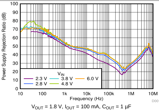
图 45. PSRR vs Frequency and V_{IN}
