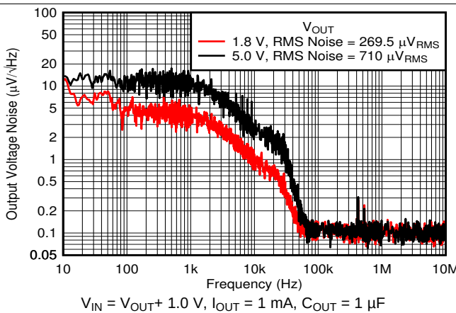
图 47. Output Noise vs Frequency and V_{OUT}
