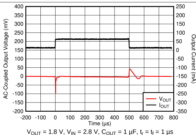
图 12. I_{OUT} Transient From 1\text{ mA} to 50\text{ mA}
