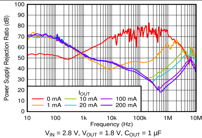
图 43. PSRR vs Frequency and I_{OUT}
