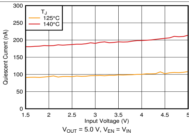
图 8. I_Q in Dropout vs V_{IN} and Temperature
