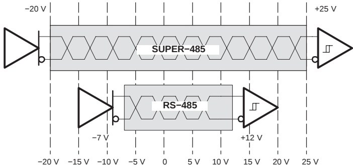
SN65HVM21 Operates Over a Wider Common-Mode Voltage Range
