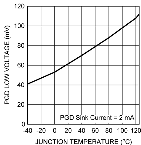
图 7-18. PGD Pin Low Voltage vs Temperature
