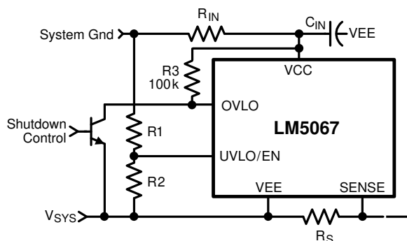
图 8-7. Shutdown/Enable Using the OVLO Pin
