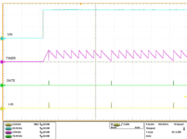
图 9-20. Power Into Short Retry Zoomed Out
