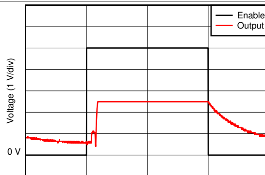
图 26. Start-Up Response
