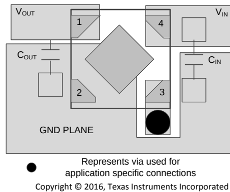
Figure 18. Recommended Layout Example
