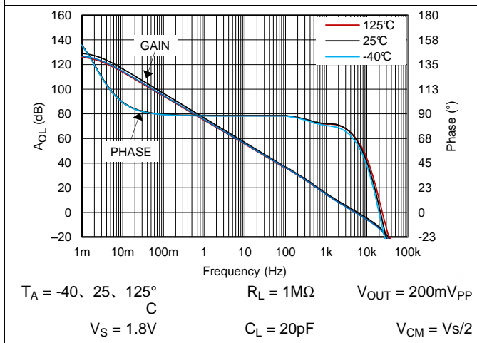
Figure 33. 开环增益和相位, 1.8V, 1MΩ 负载
