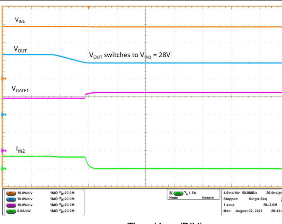
图 9-15. ORing V_{IN2} to V_{IN1} Switch Over
