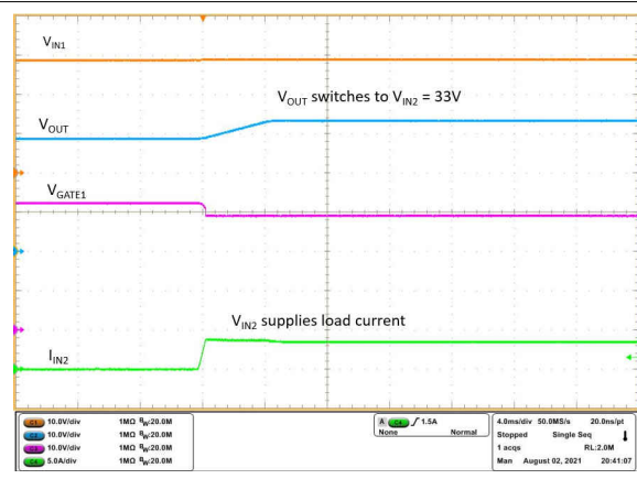
图 9-13. ORing V_{IN1} to V_{IN2} Switch Over
