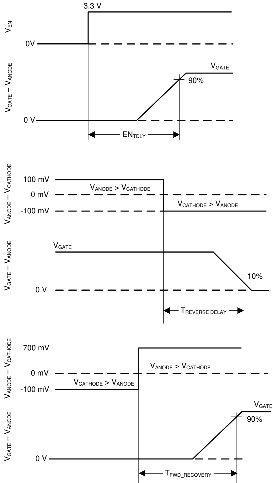
图 7-1. Timing Waveforms
