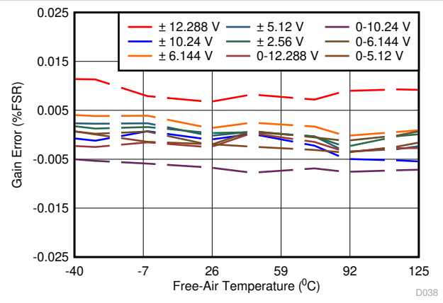
图 6-30. Gain Error vs Temperature Across Input Ranges
