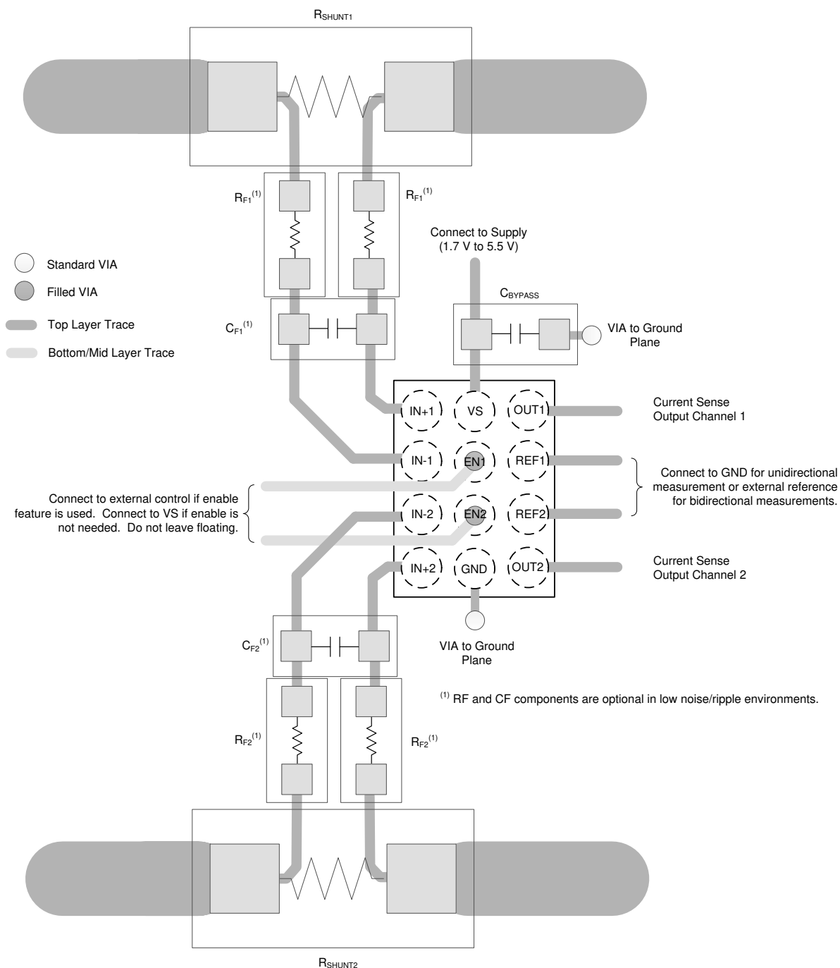
图 10-2. Recommended Layout Dual Channel DSBGA (YBJ) Package
