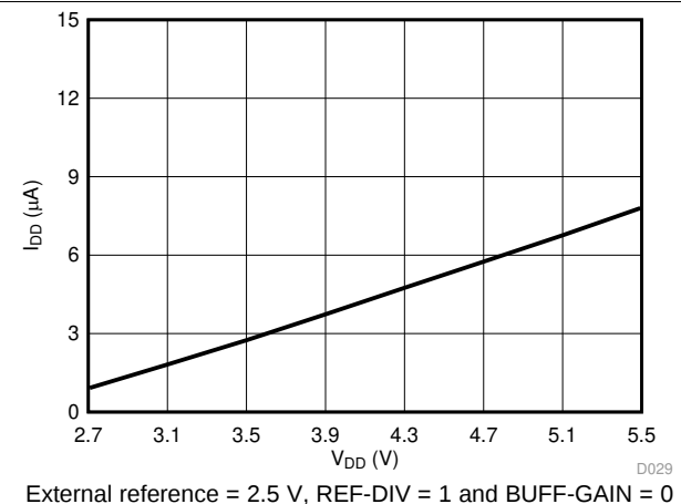
图 31. Power Down Current vs Supply Voltage
