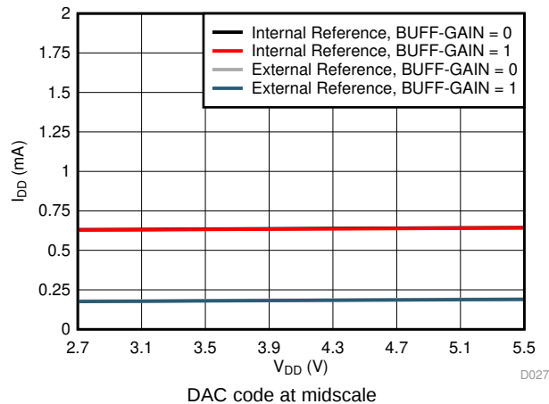
图 29. Supply Current vs Supply Voltage
