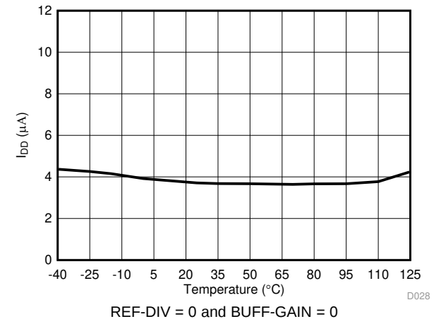
图 30. Power Down Current vs Temperature
