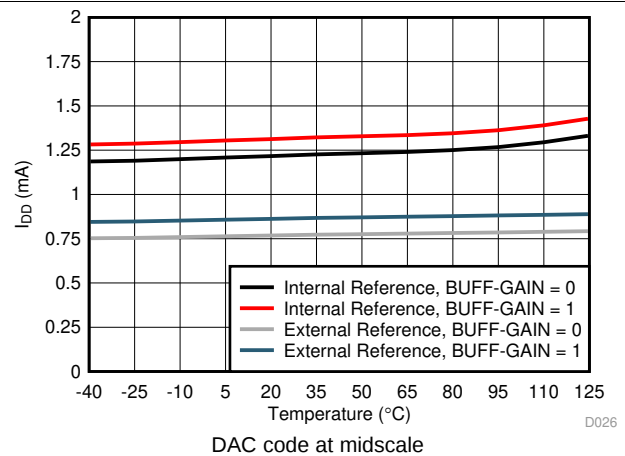
图 28. Supply Current vs Temperature
