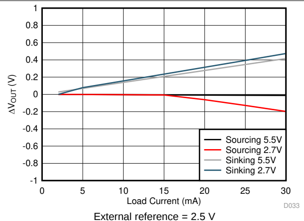
图 32. Headroom and Footroom vs Load Current
