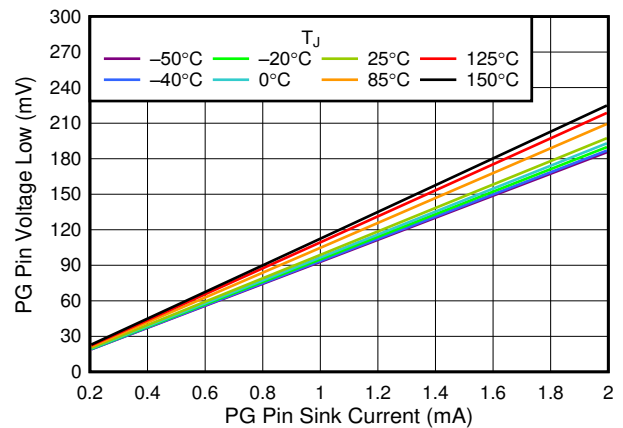
图 6-22. V_{OL}(PG) vs PG Pin Sink Current
