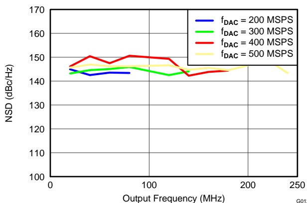
Figure 12. DAC3154 NSD vs Output Frequency Over f_{DAC}
