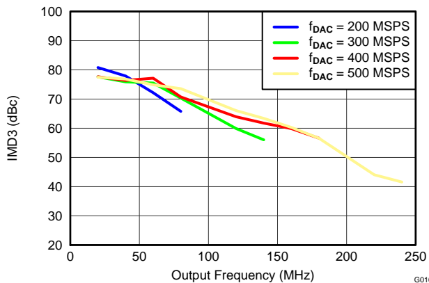
Figure 10. DAC3154 IMD3 vs Output Frequency Over f_{DAC}
