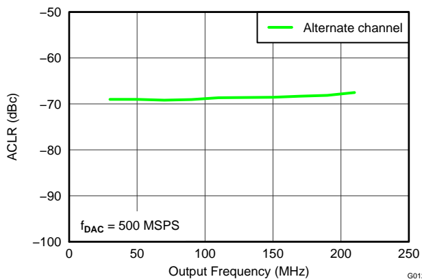
Figure 14. DAC3154 ACLR (Alternate Channel) vs Output Frequency
