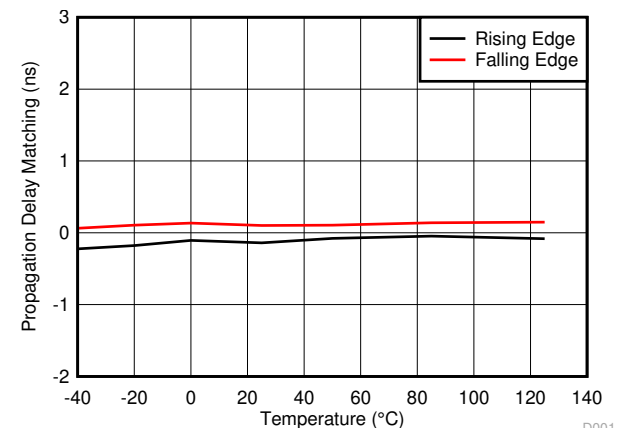
Figure 7-19. Propagation Delay Matching, Rising and Falling Edge
