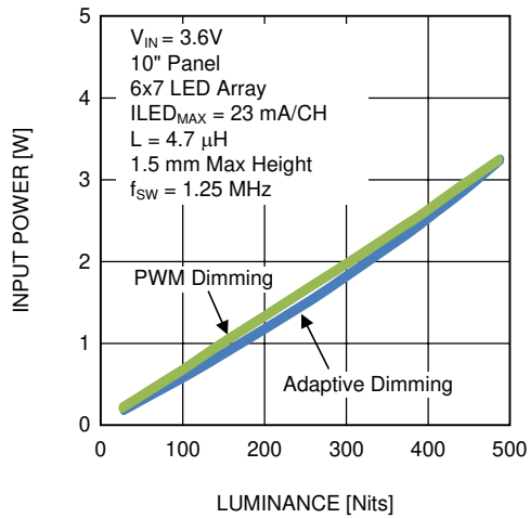
Figure 26. Input Power as a Function of Brightness
