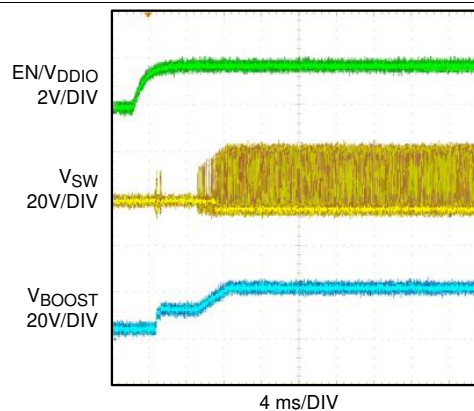
Figure 3. Start-Up Waveforms
