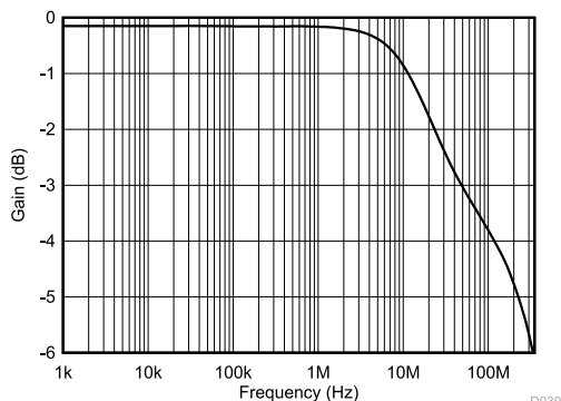
图 7-25. On Response vs Frequency
