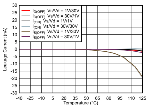
图 7-9. Leakage Current vs Temperature
