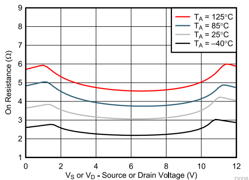
图 7-7. On-Resistance vs Temperature
