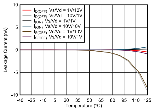
图 7-10. Leakage Current vs Temperature
