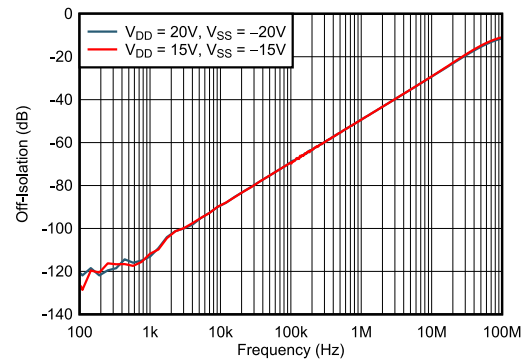
图 7-20. Off-Isolation vs Frequency
