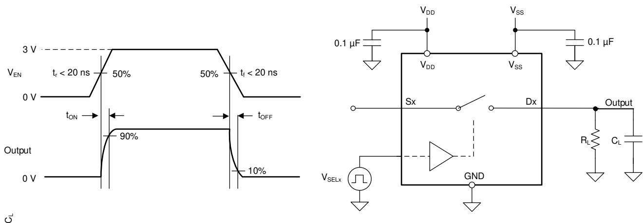
图 8-4. Turn-On and Turn-Off Time Measurement Setup
