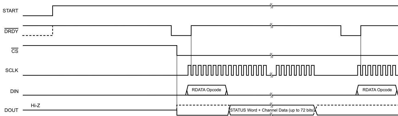
Figure 53. RDATA Usage
