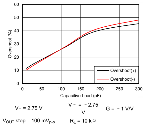
图 8-24. Small-Signal Overshoot vs Load Capacitance
