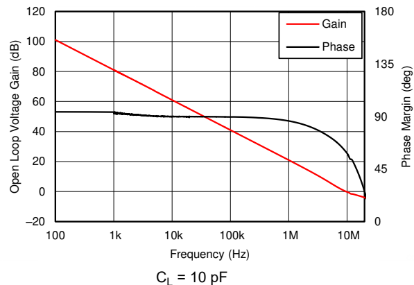
图 8-6. Open-Loop Gain and Phase vs Frequency
