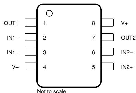
图 7-2. TLV9062-Q1 D, DGK, and PW Package 8-Pin SOIC, VSSOP, and TSSOP Top View
