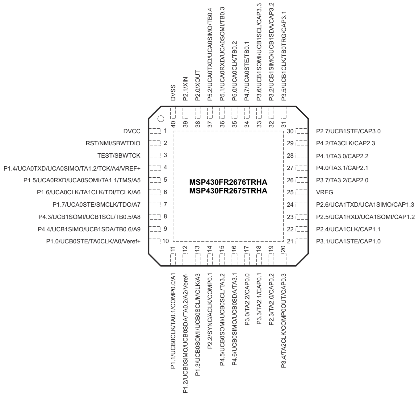
图 7-2. 40-Pin RHA Package (Top View)
