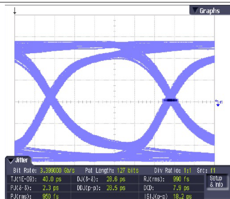
Figure 21. SN75DP126 Output; 22-inch Input Trace; 15 dB EQ Setting; TMD5 Sink
