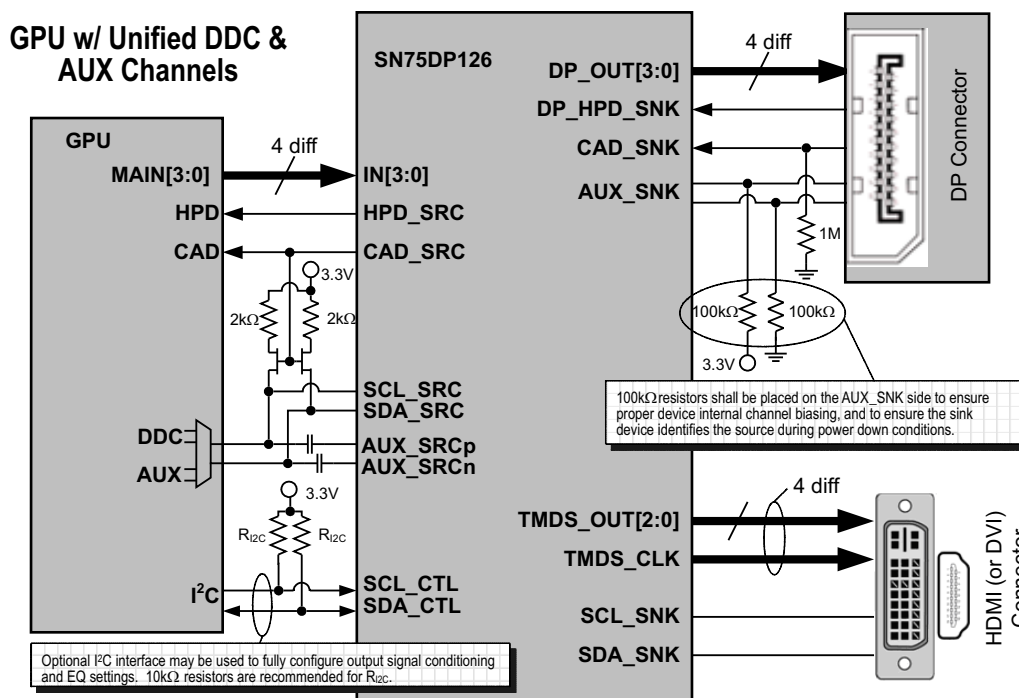
Figure 24. GPU with a Unified AUX/DDC Configuration
