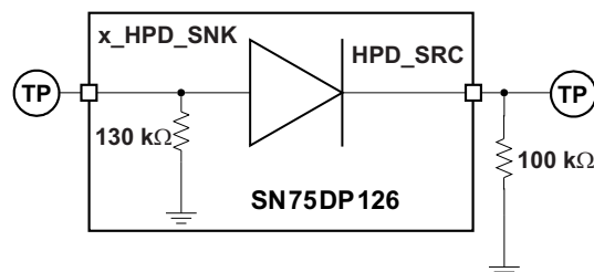
Figure 6. HPD Test Circuit
