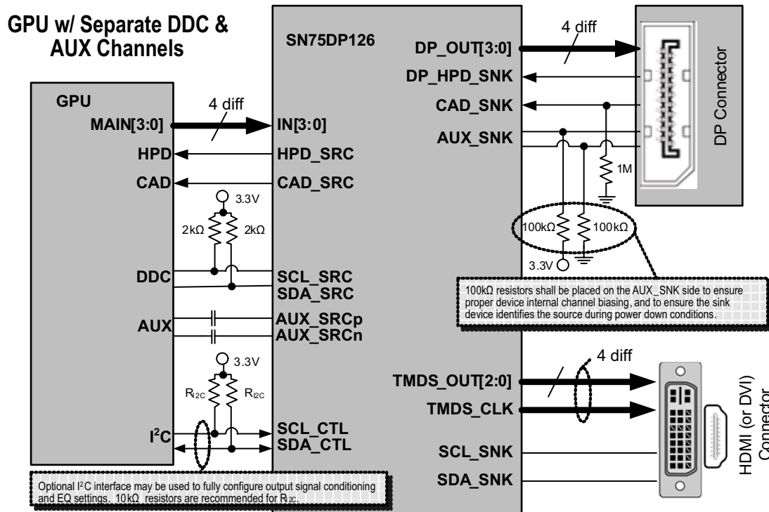
Figure 25. GPU with Separate DDC and AUX Channels
