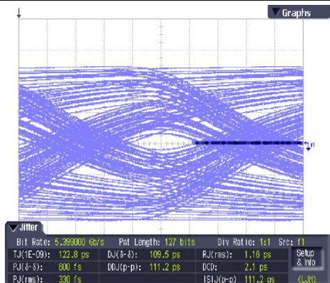
Figure 32. Main Link Input with 22-inch Trace; DisplayPort Sink
