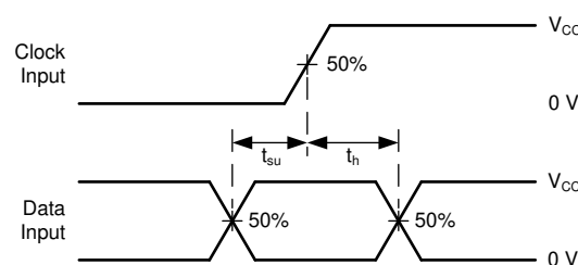
Figure 7-4. Voltage Waveforms, Setup and Hold Times
