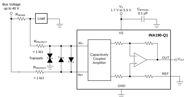
图 37. Transient Protection Using a Single Transzorb and Input Clamps
