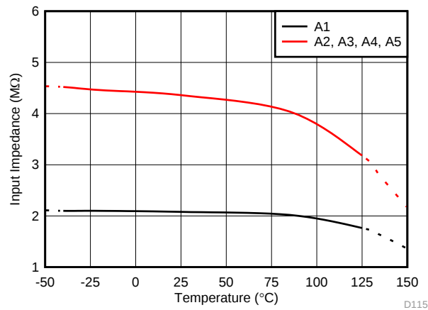
图 35. Differential Input Impedance vs Temperature
