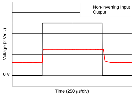
图 21. Common-Mode Voltage Transient Response
