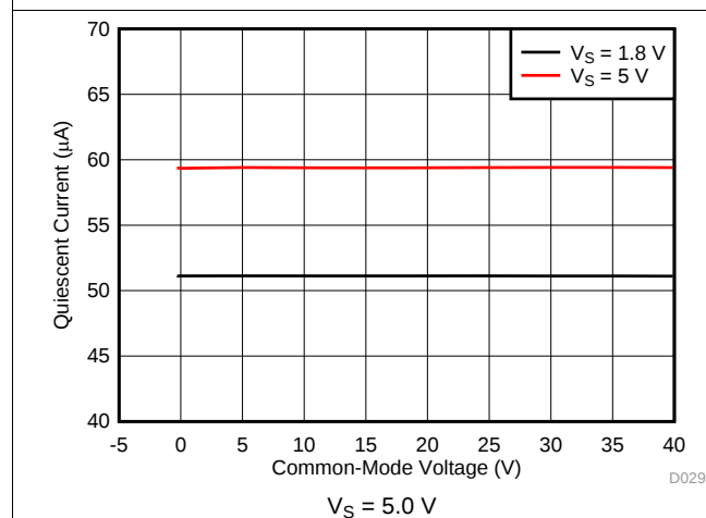
图 17. Quiescent Current vs Common Mode Voltage
