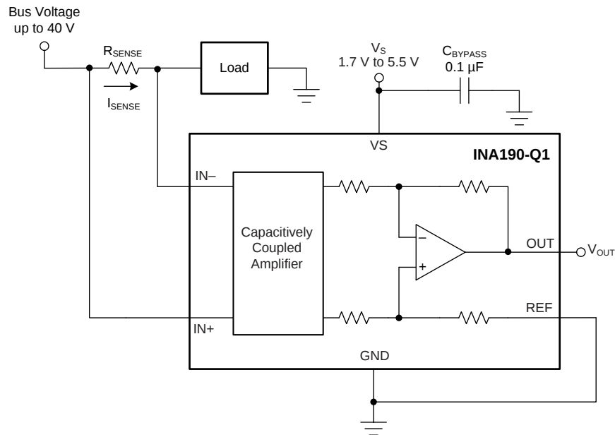
图 30. Typical Unidirectional Application
