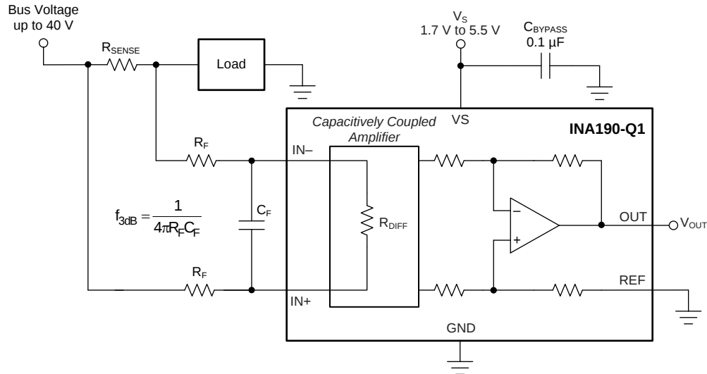
图 34. Filter at the Input Pins
