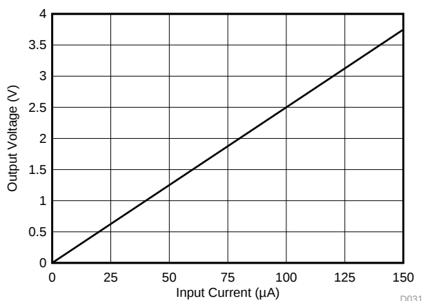
图 39. Typical Application DC Transfer Function
