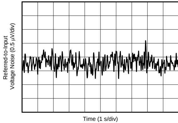
图 19. 0.1-Hz to 10-Hz Voltage Noise (Referred-To-Input)
