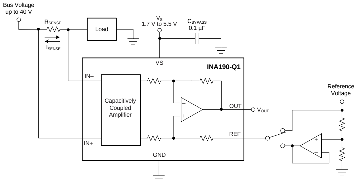
图 32. Bidirectional Application
