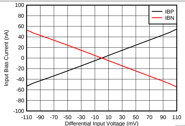
图 26. IB+ and IB- vs Differential Input Voltage
