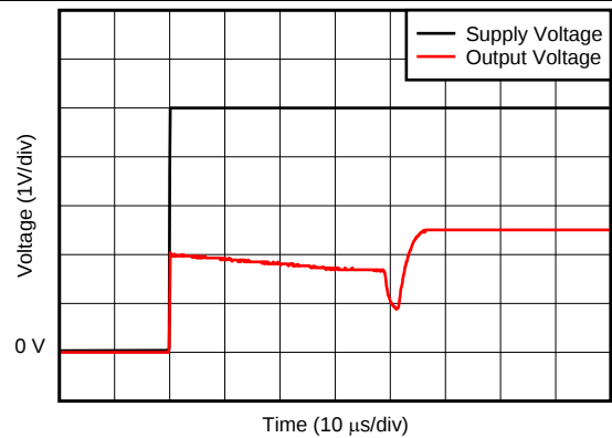
图 22. Inverting Differential Input Overload
