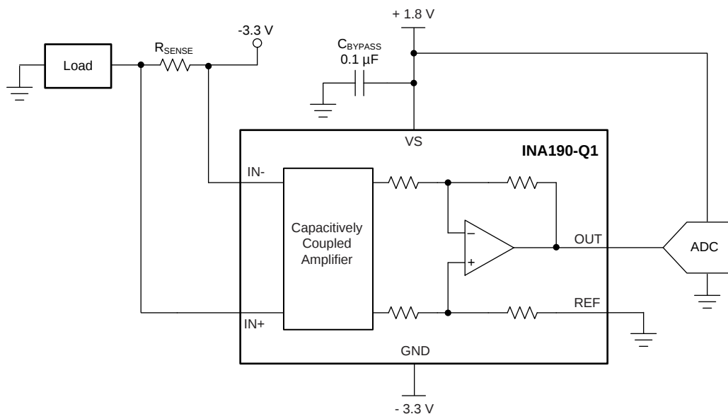
图 31. Using the REF Pin to Level-Shift Output Voltage
