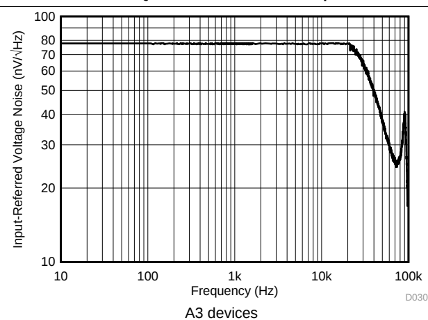
图 18. Input-Referred Voltage Noise vs Frequency
