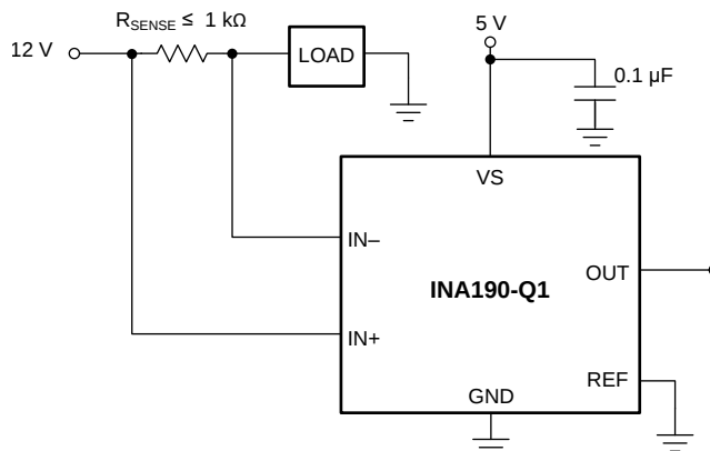
图 38. Microamp Current Measurement
