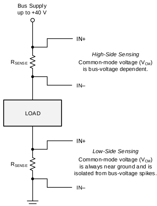
图 29. High-Side and Low-Side Sensing Connections
