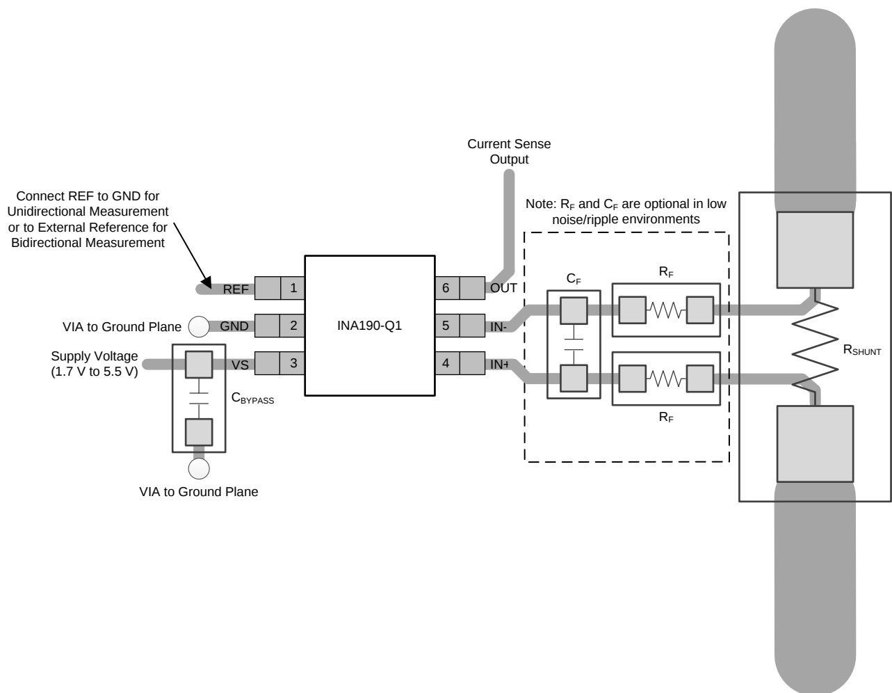
图 40. Recommended Layout for SC70 (DCK) Package
