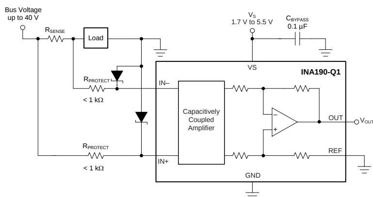
图 36. Transient Protection Using Dual Zener Diodes
